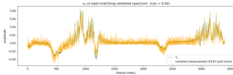
Figure 6: The leading eigenvector \mathbf{v}_1 (green) overlaid on the best-matching centred spectrum (cosine \approx 0.92 ). It reads as a difference spectrum supported on two molecular bands.
