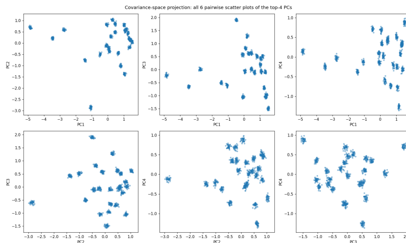
Figure 7: The six pairwise scatter plots of the top-four covariance scores. Each point is a vial; the data resolves into about 25 clusters.
